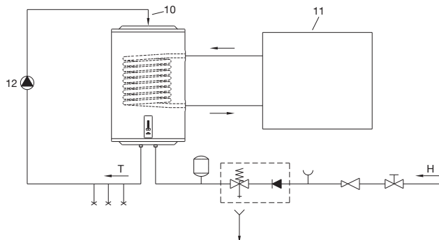
Fig. 4: Connection to alternative sources of heating
