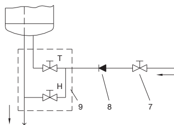
Fig. 3: Open (non-pressure) system
