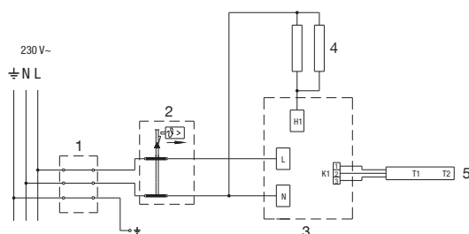
Fig. 6: Electric installation
