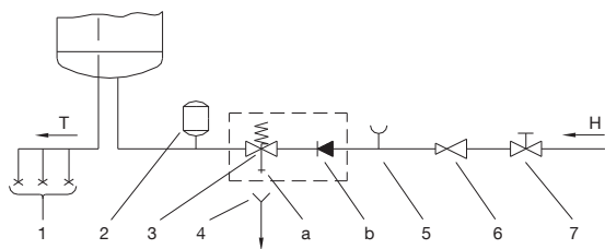
Fig. 2: Closed (pressure) system
