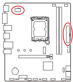
CPU_PWR1
