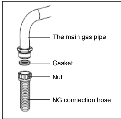
NG Connection
