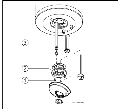
Fig. 14 Access to the interior and component identification
