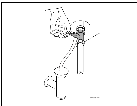
Fig. 8 Opening the pressure relief valve
