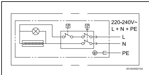
Fig. 17 Connection diagram
